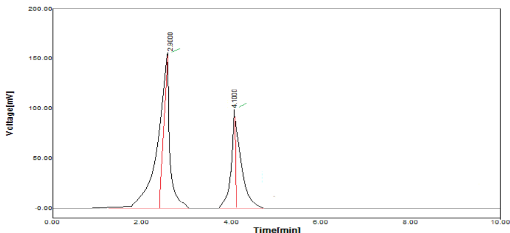
Fig 3: Representative Chromatogram for Resveratrol and Curcumin combination by HPLC
