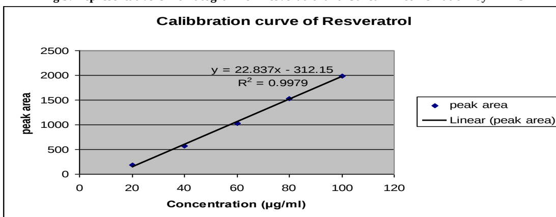
Fig :4 Calibration curve indicating linearity range of Resveratrol by HPLC
