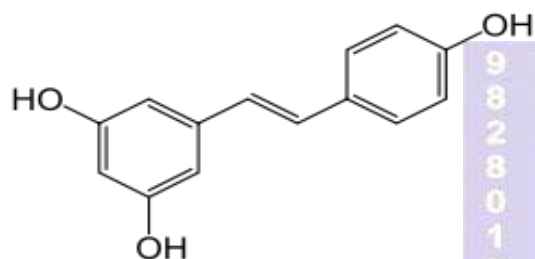
Fig: 1 structure of Resveratrol
