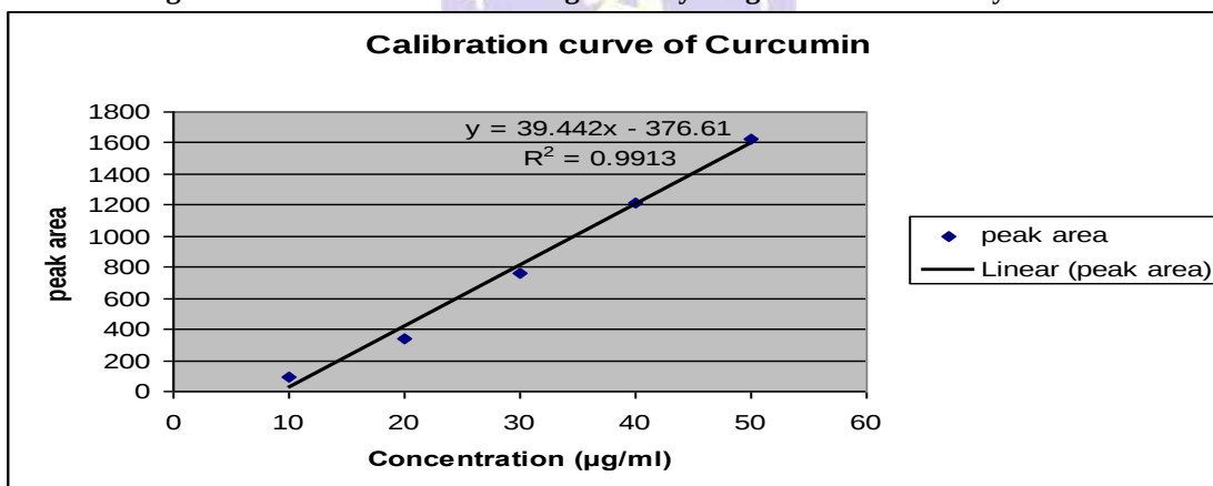
Fig 5: Calibration curve indicating linearity range of Curcumin by HPLC
