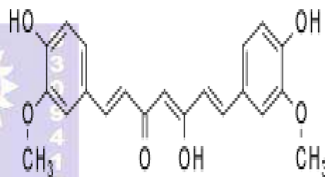
Fig:2 structure of Curcumin
