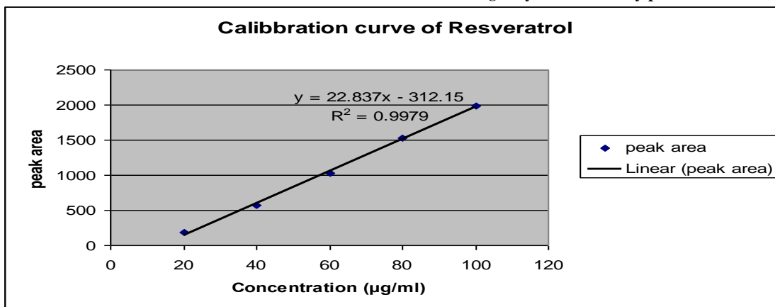
Fig 6 Calibration curve indicating linearity range of Resveratrol by HPLC
