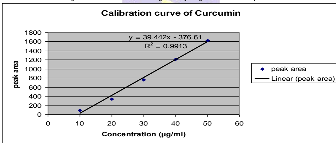
Fig 7 :Calibration curve indicating linearity range of Curcumin by HPLC
